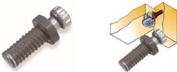
ONE-SIDED DOWEL
